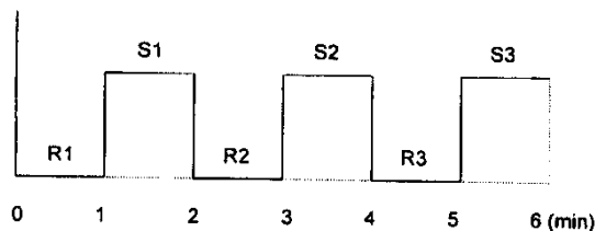
图 1. fMRI 刺激模式示意图 Fig. 1. Stimulation paradigm. R1, R2, R3 represent the resting phases without TENS stimulation and S1, S2, S3 the TENS stimulating phases.
